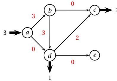
Fig. 9.6 The result of augmenting a flow of one along the negative cycle in Figure 9.4. This flow has cost 12 but is not optimal, since the residual network still contains a negative cycle.
