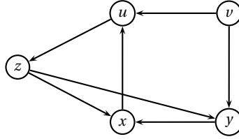
Fig. 9.1 Example of a directed graph with 5 nodes and 7 arcs.
