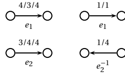
Fig. 9.5 Two arcs e_1, e_2 \in A labeled with f(e)/f^\circ(e)/u(e) and the corresponding flow on these arcs (or their reverse) in D(f^\circ) . Arcs in D(f^\circ) are labeled with flow and capacity values respectively.
