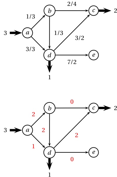
Fig. 9.3 A Network with in/out-flow, costs and capacities and a feasible flow of cost 13.
